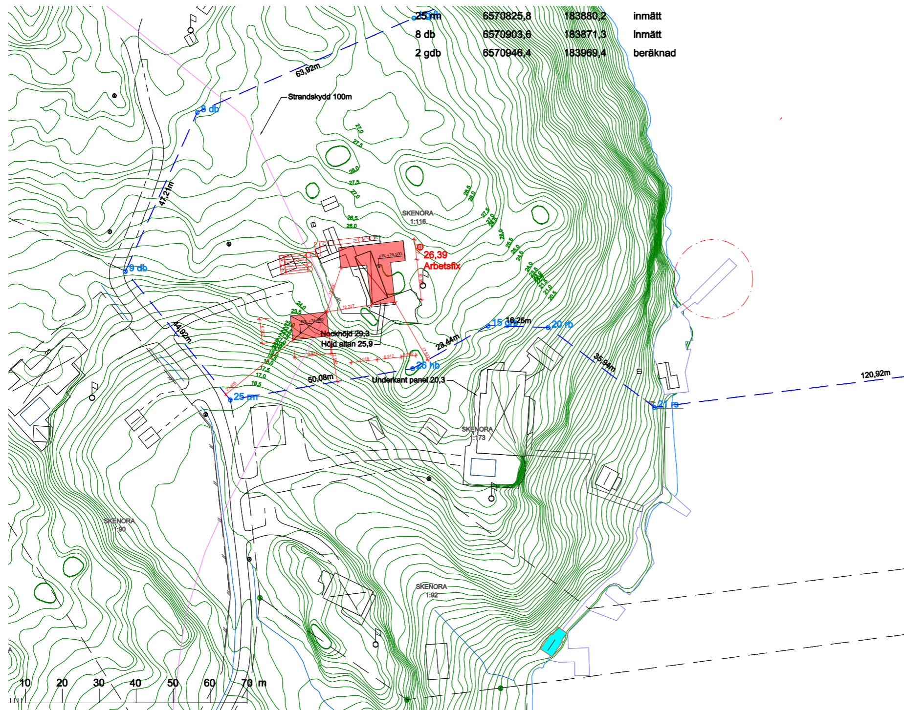
Situationsplan 1:1000
